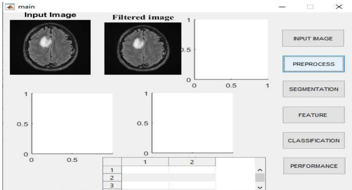
Fig 5 filtered mage
