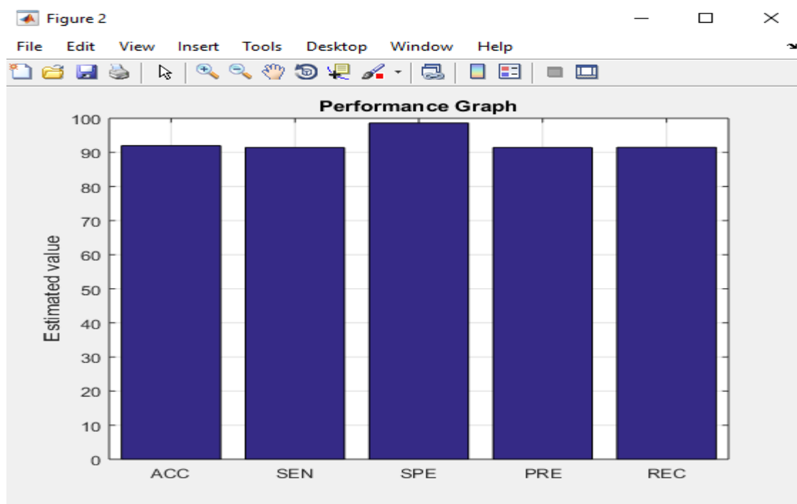
Fig.8 performance graph
