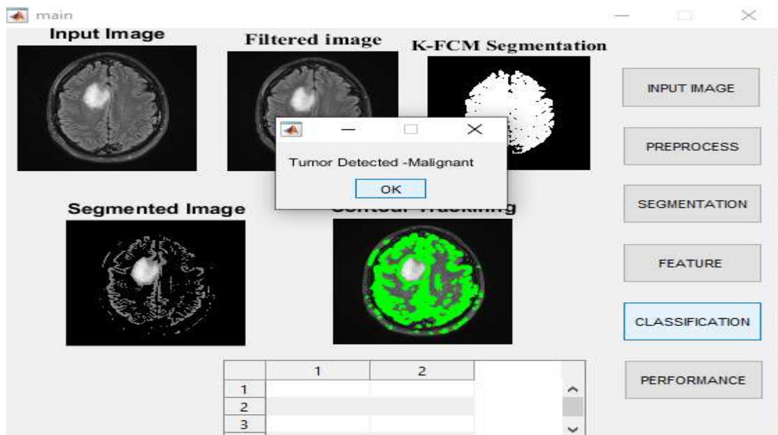
Fig.7 Tumor Classification
